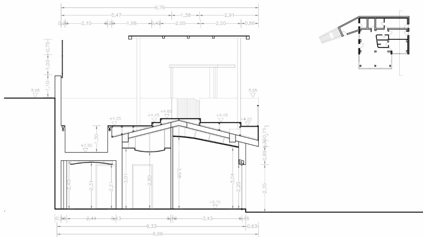
Section C-C' 1:50
