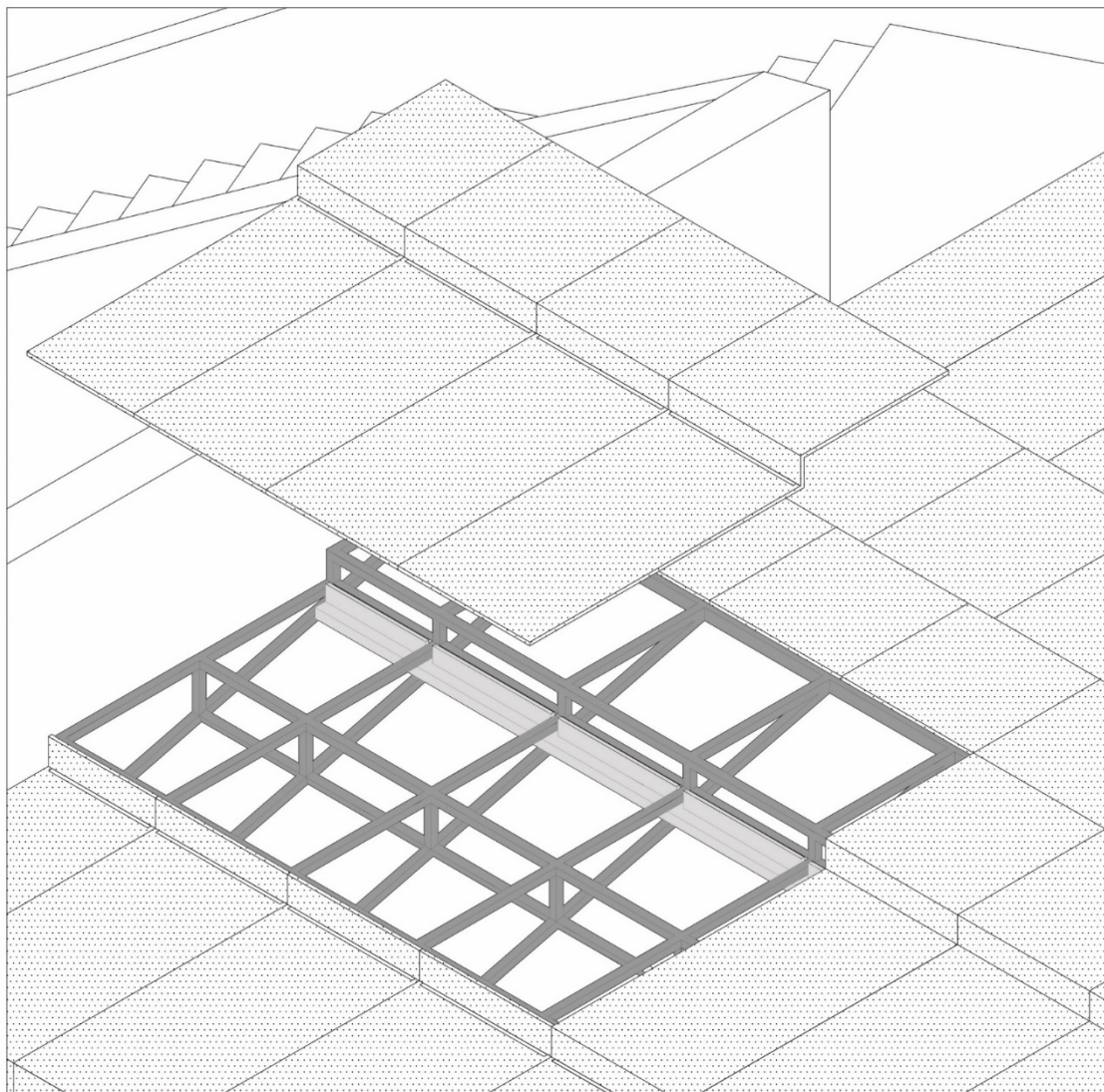
Roof Detail
